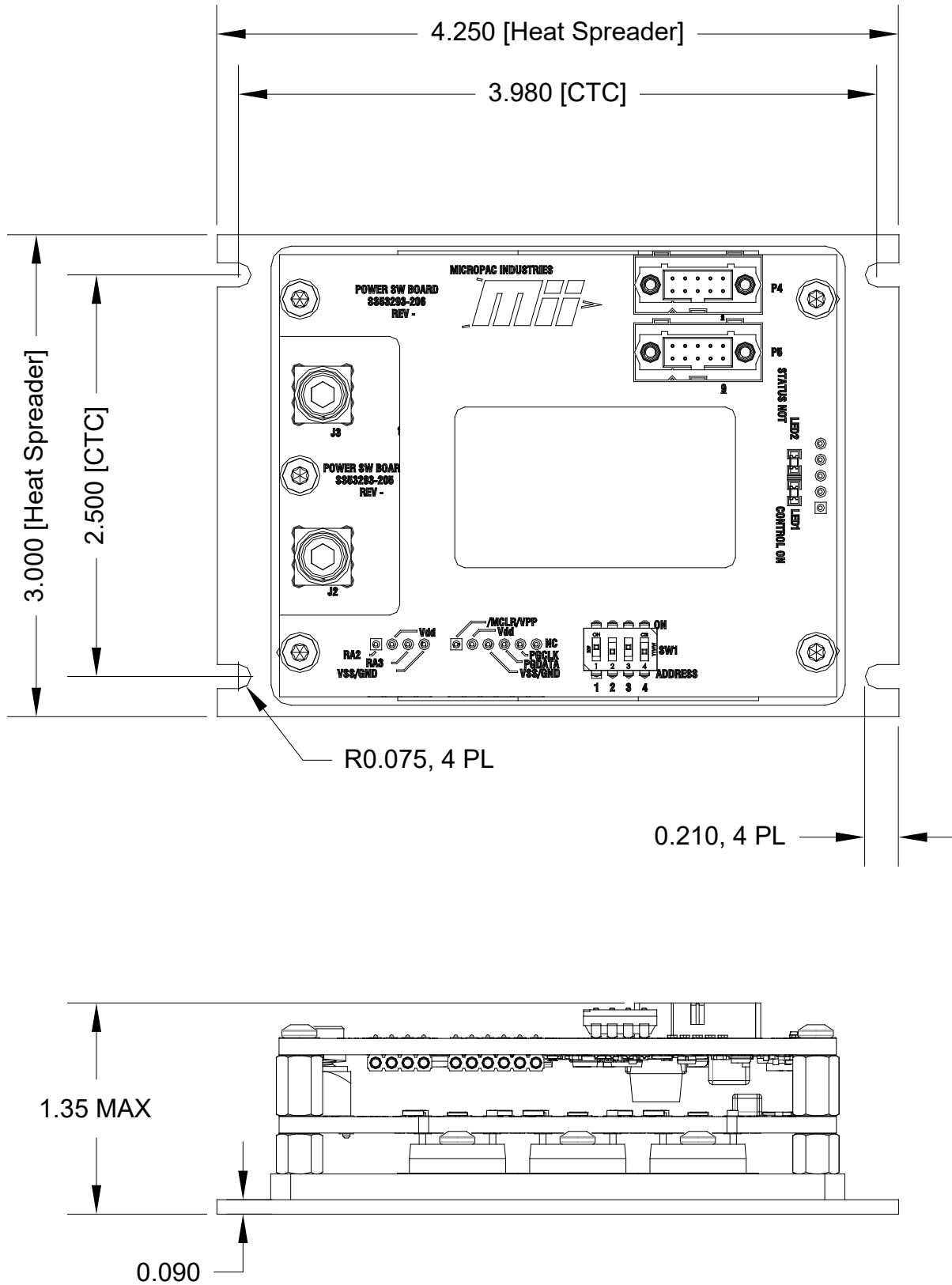
Figure 5 Package Dimensions
