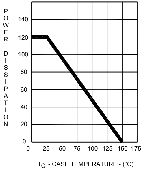
Figure 1. Power Derating
